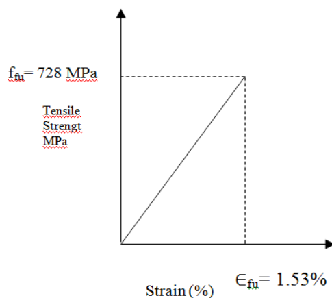
Figure 6 Elastic stress strain curve of GFRP used
