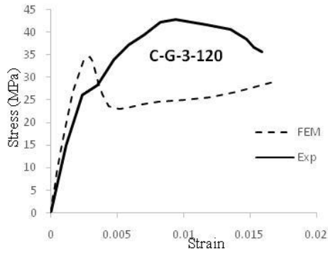
Figure 7 Numerical and Experimental Stress Versus Strain Behavior for Concentrically Loaded GFRP and Steel Reinforced Columns
