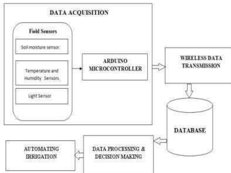
Fig.1: System Design
