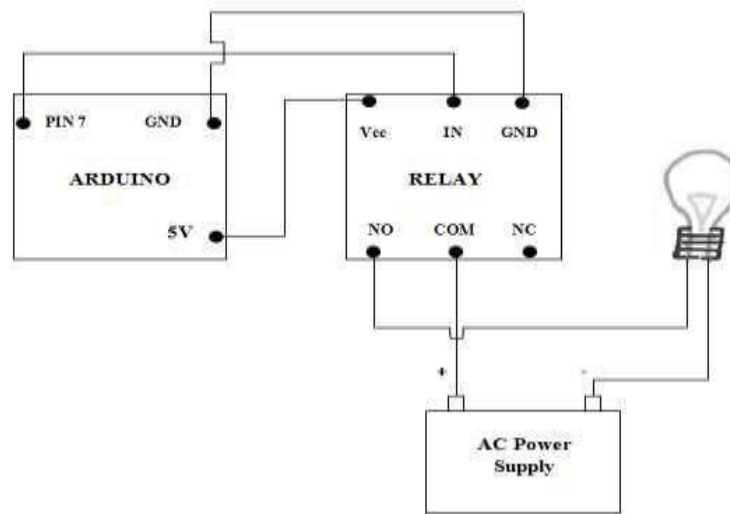
Fig. 7: Connection of Relay with Arduino and AC Power Supply
