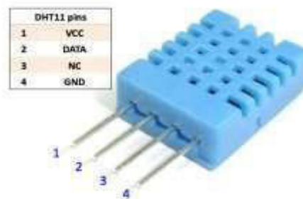
Fig. 3: DHT11 Temperature and humidity Sensor
