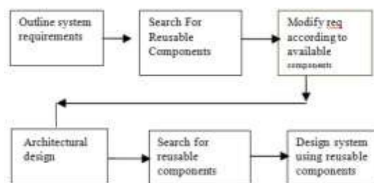
Fig. 1 Software process using reusable artifacts
