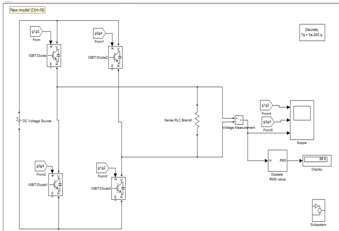
Figure 9-Two level inverter
