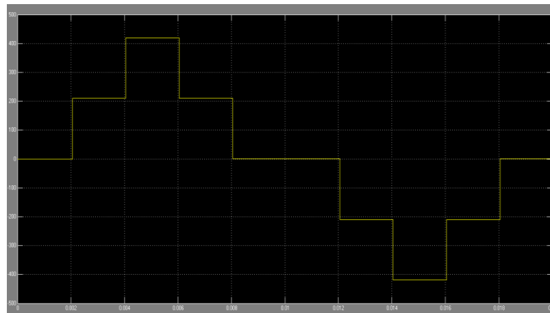
Figure 16-Seven level cascaded inverter output voltage
