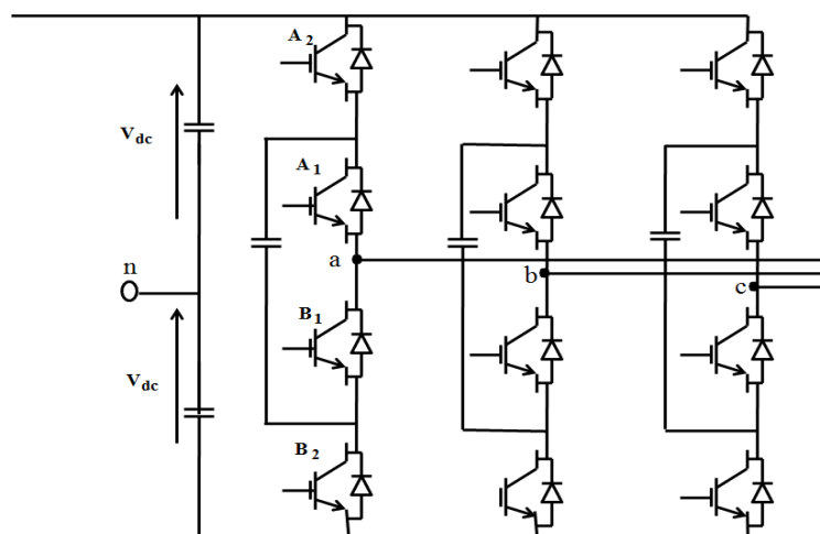
Figure 5- A flying capacitor clamped MLI
