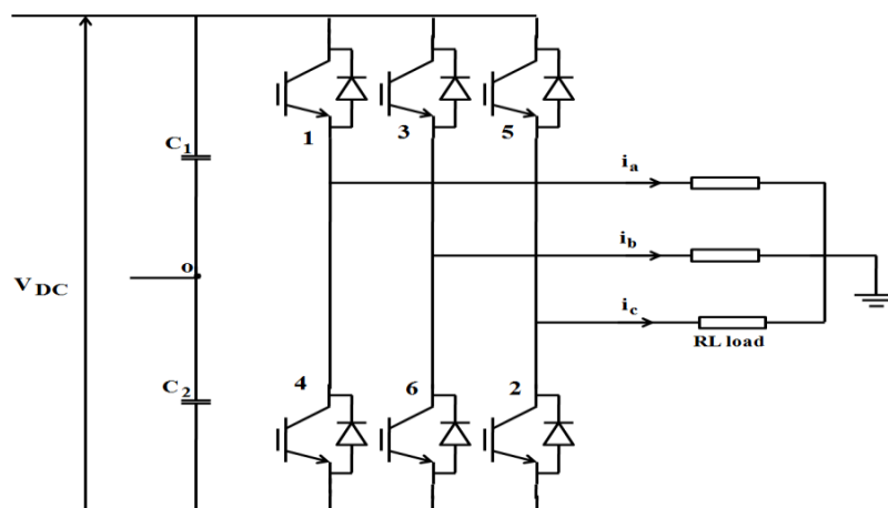
Figure 1- One phase leg of a two-level inverter, two level output wave form without PWM
