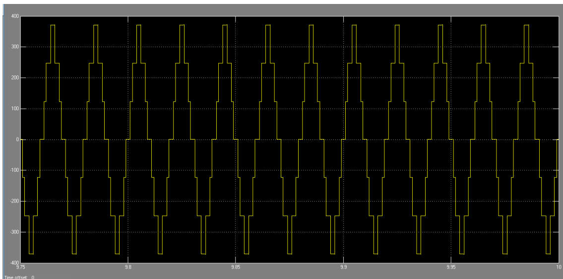
Figure 19-Seven level MLI
