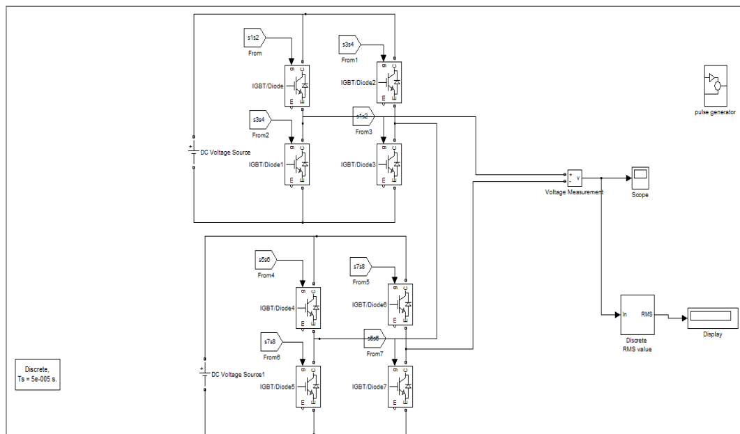
Figure 12-Five level cascaded inverter
