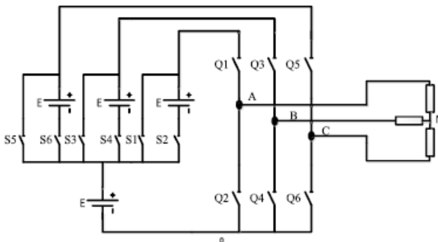
Figure 8 – Proposed three-phase MLI topology
