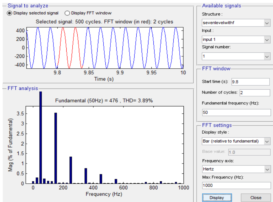
Figure 22- FFT analysis
