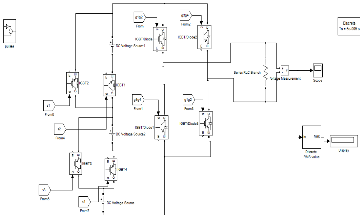
Figure 18-Seven level MLI
