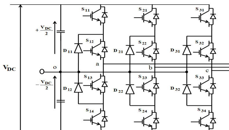
Figure 2- Single leg of a three-level inverter
