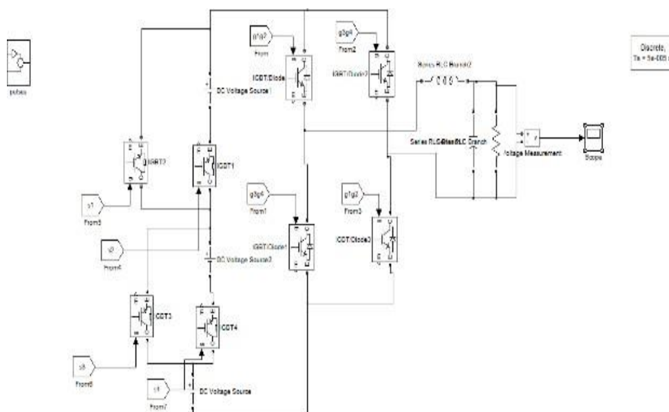
Figure 21-proposed 7level MLI with filter
