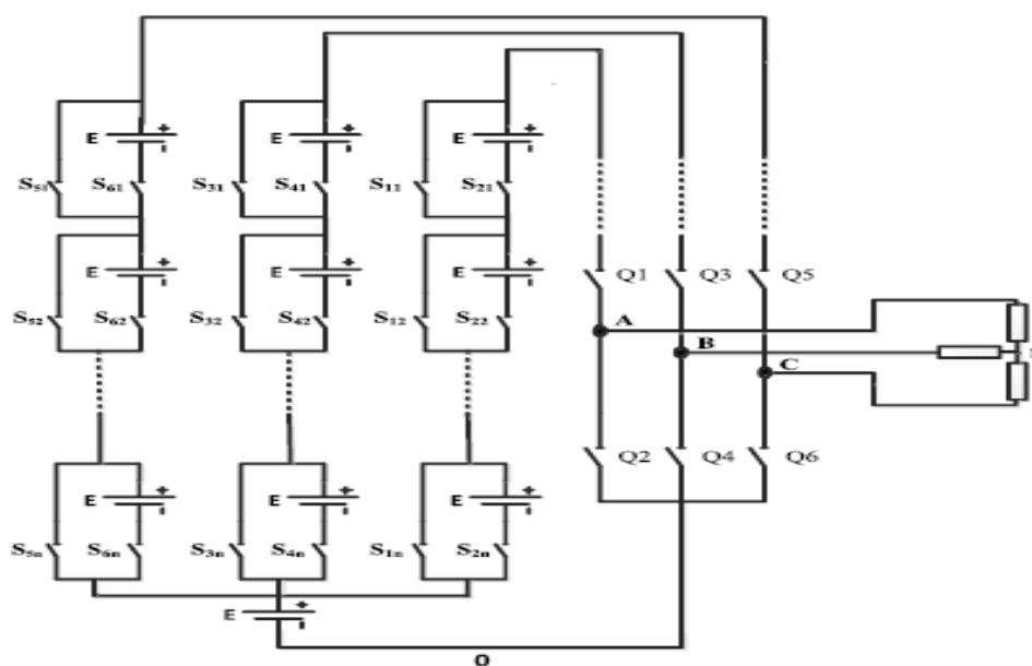
Figure 7 – Power circuit of the three-phase MLI
