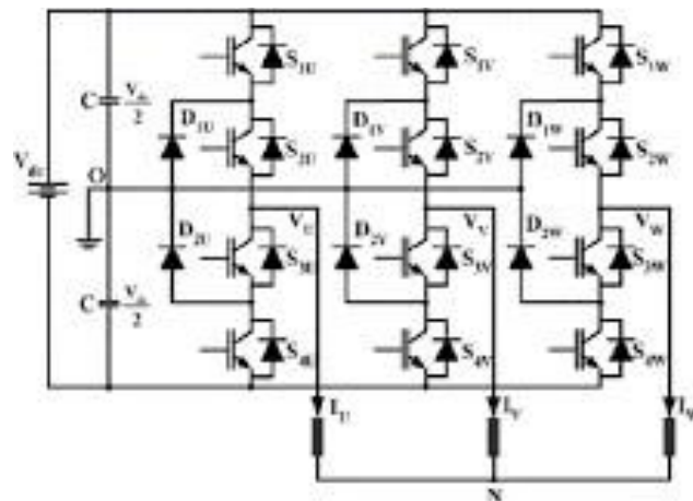
Figure 4- A Five level diode clamped MLI
