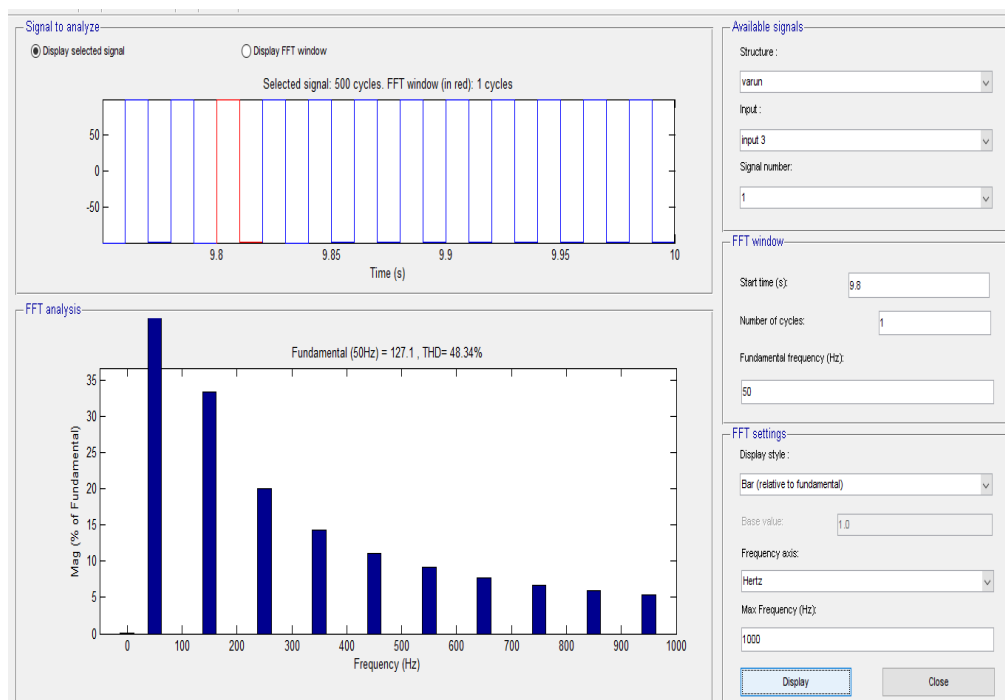
Figure 11-FFT analysis
