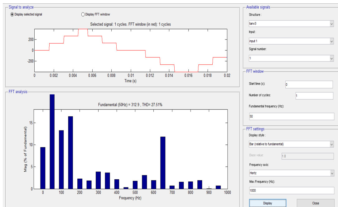
Figure 17-FFT analysis
