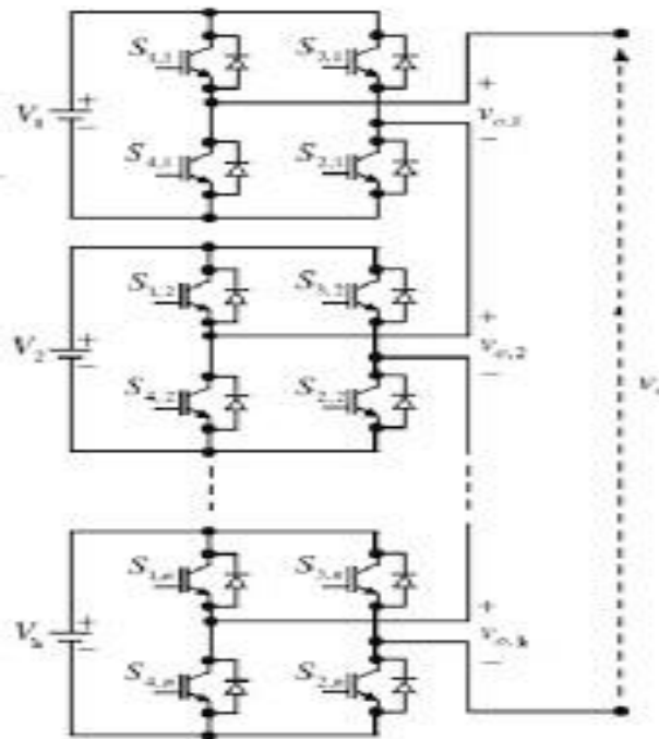
Figure 6- A 5 level H-bridge inverter
