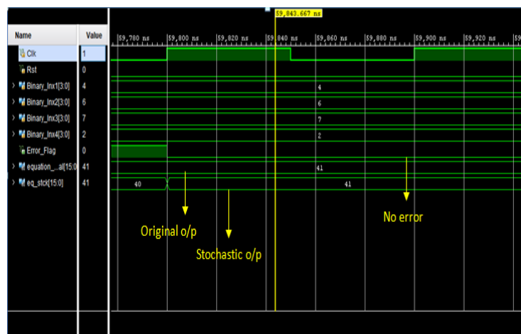
Fig.9. Equation simulation window
