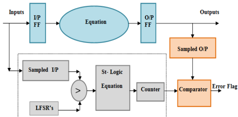
Fig.4. Stochastic checker for equation
