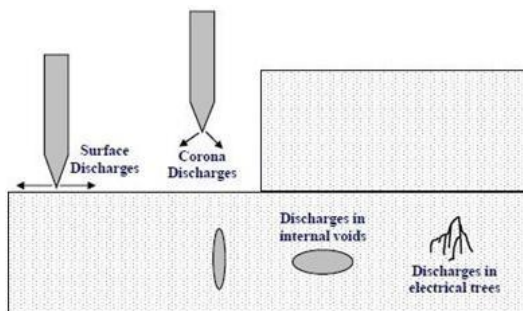
Figure 2: Different types of discharges
