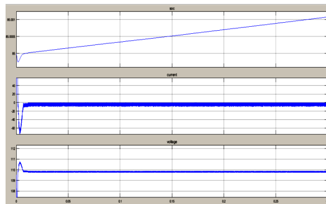
Figure 6: Battery (SOC, Current, Voltage)
