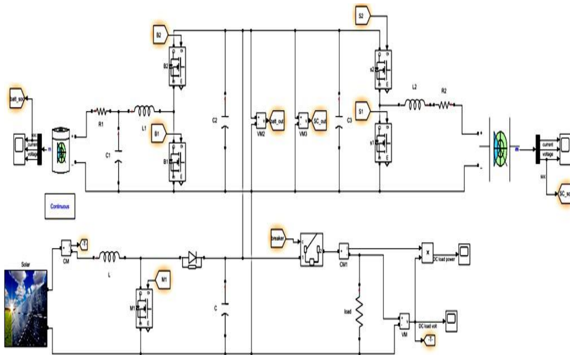
Figure 2: Proposed Model
