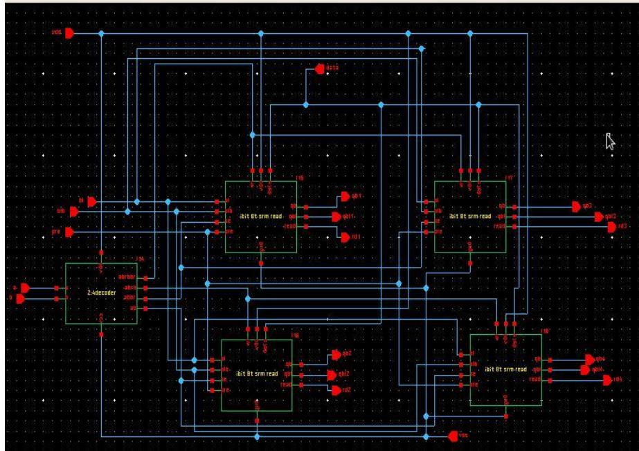
Fig 5: Proposed 8T 4 bit SARM memory unit
