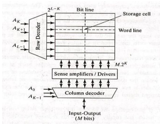
Fig 4: basic memory block
