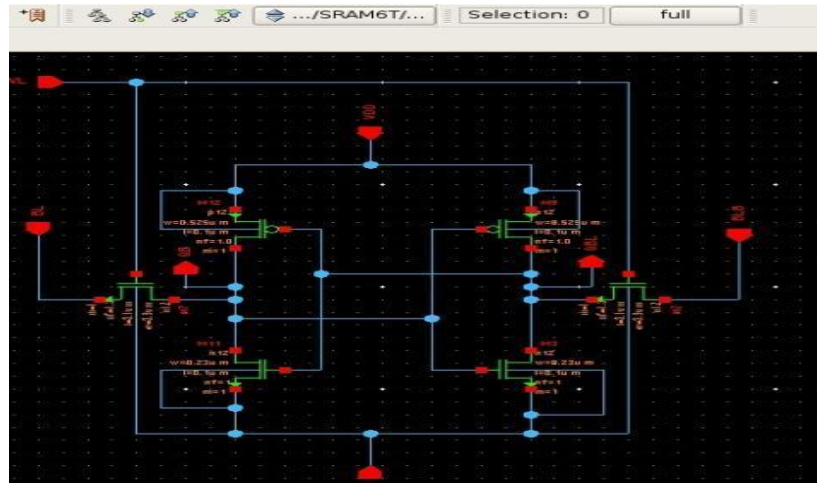
Fig 2: Conventional 6T SRAM
