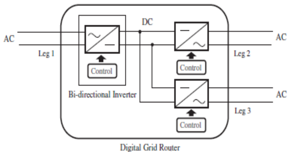
Fig.3. Digital grid router with VSC
