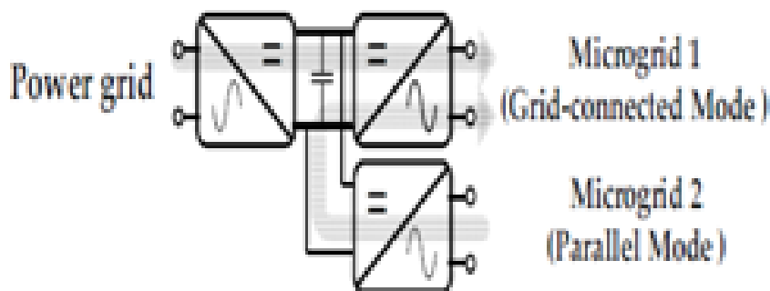
Fig.8. Power flow from main grid and micro grid2 to micro grid 1
