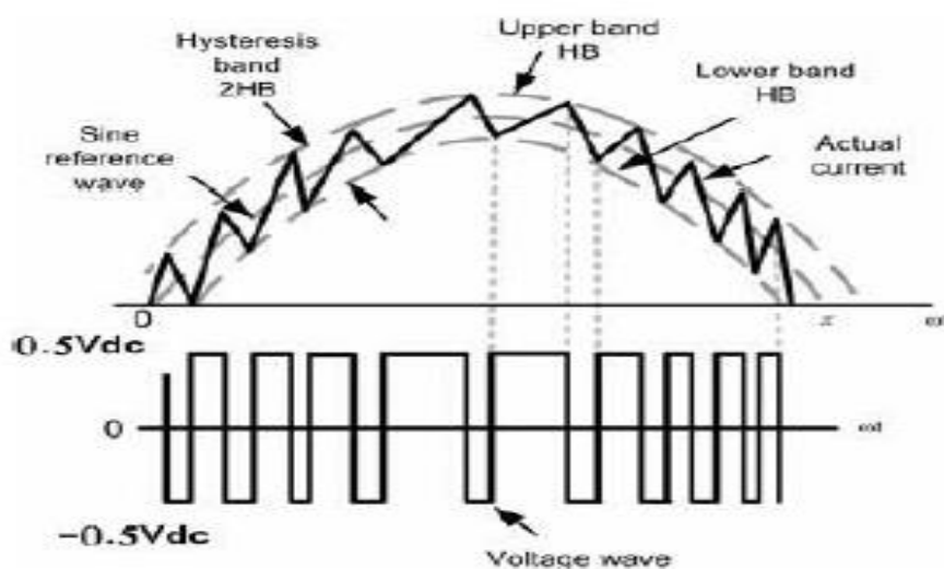
Figure: - 4 Hysteresis control method
