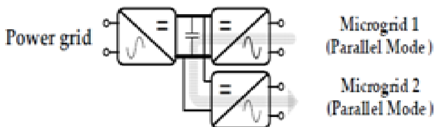
Fig.10. Power flow from micro grid 1 to micro grid 2
