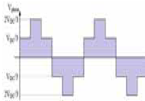
Fig.5. Output voltage waveform of hysteresis control converter
