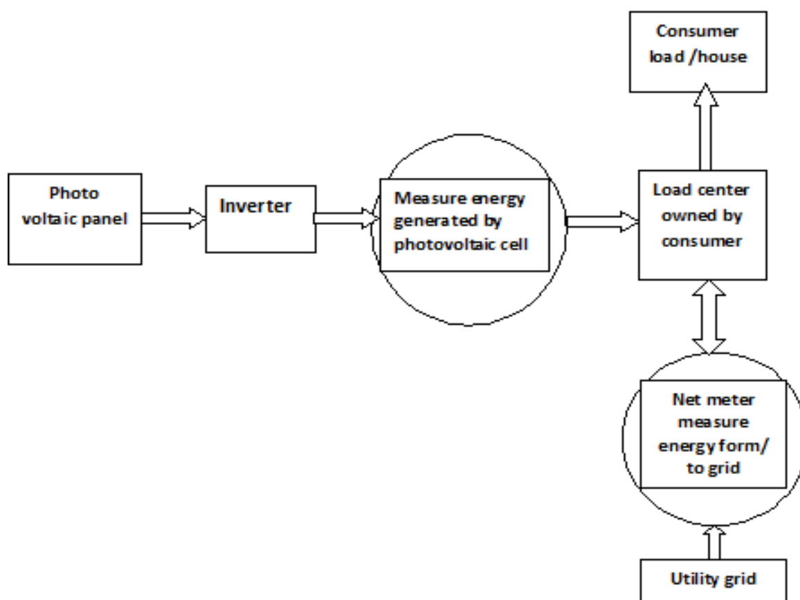
Fig.11. block diagram of bi-directional energy meter
