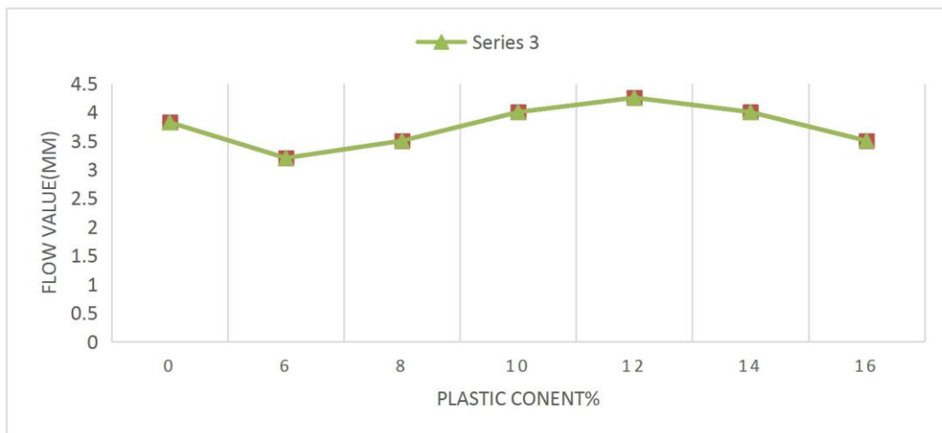
Figure 6: Variations pf plastic content to the flow value
