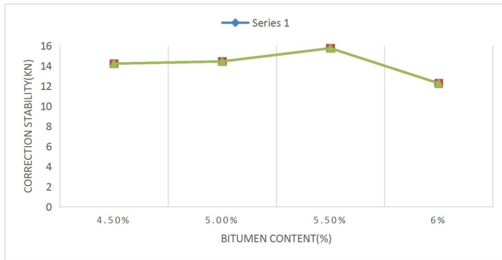
Figure 1: Variations of stability to the bitumen content
