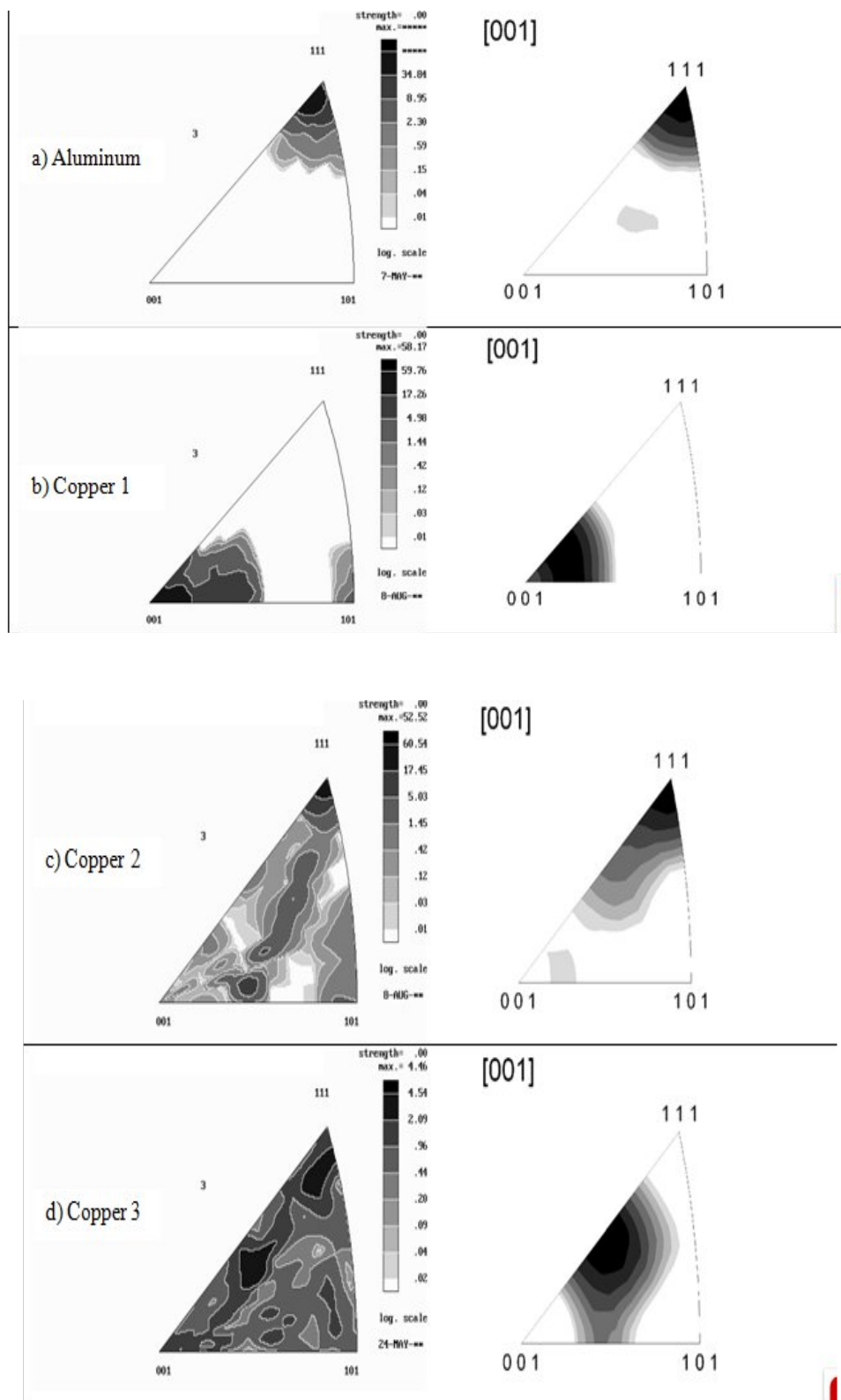
Figure.3 Comparison of inverse pole figure generated by XRD (left) and EBSD (right). See Table 1 for sample details.
