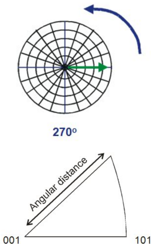
Fig. 2 Construction of direct (left) and inverse (right) pole figures. A direct pole figure shows only information for one crystallographic direction. Combining the information from several pole figures of crystallographically independent directions will yield an inverse pole figure, which normally is a more useful presentation, especially for thin films.
