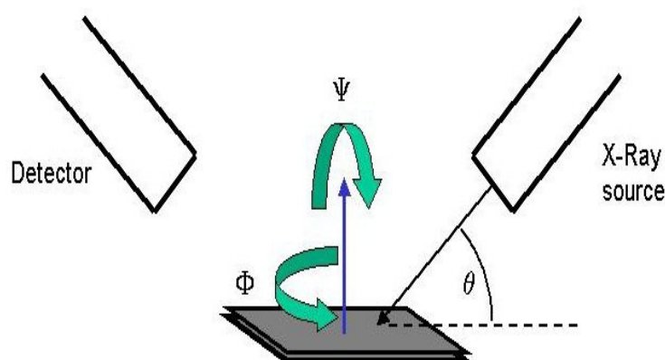
Fig. 1 (a) Pole figure measurement by XRD. 2\theta : Diffraction angle; \psi : Rotation angle; \phi : Tilt angle.
