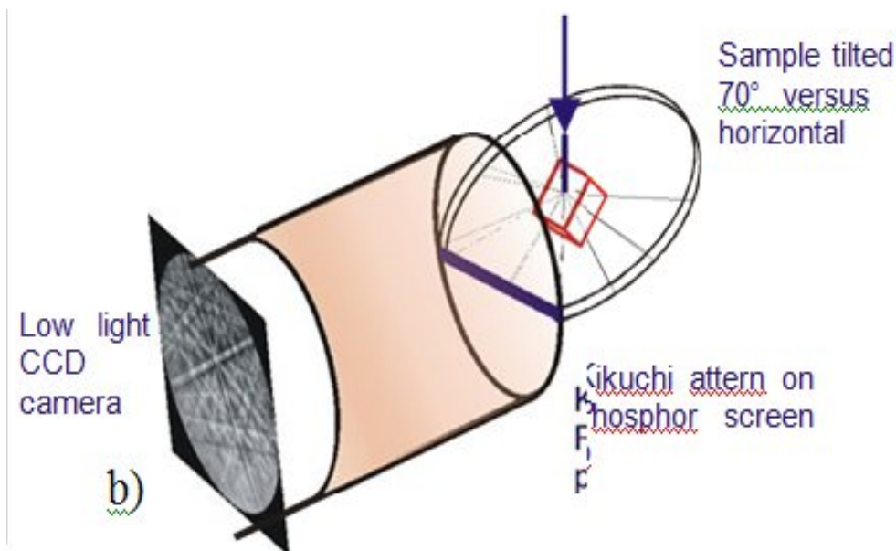
Figure 1 (b) Principle of an EBSD measurement.
