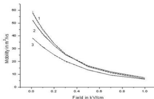
Fig. 2: Variation of Electron Mobility with Applied Electric Field at 77 K for InSb at Different Ionized Impurity Concentrations (1) N_i = 0 , (2) N_i = 1e14 , (3) N_i = 5e14
