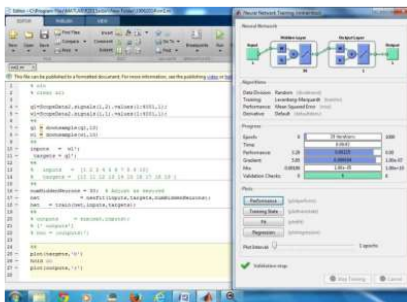
Figure 7. Training of Proposed NNC
