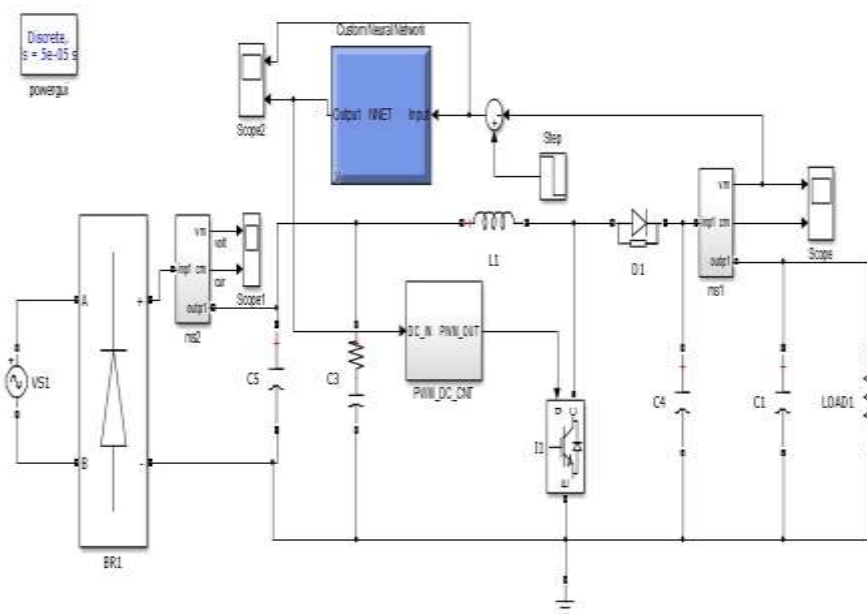
Figure 4. Neural Network Controller for DC-DC (Buck) Power Converter Circuit
