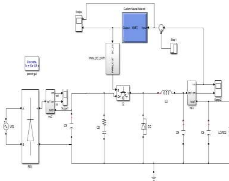
Figure 5. Neural Network Controller for DC-DC (Boost) Power Converter Circuit
