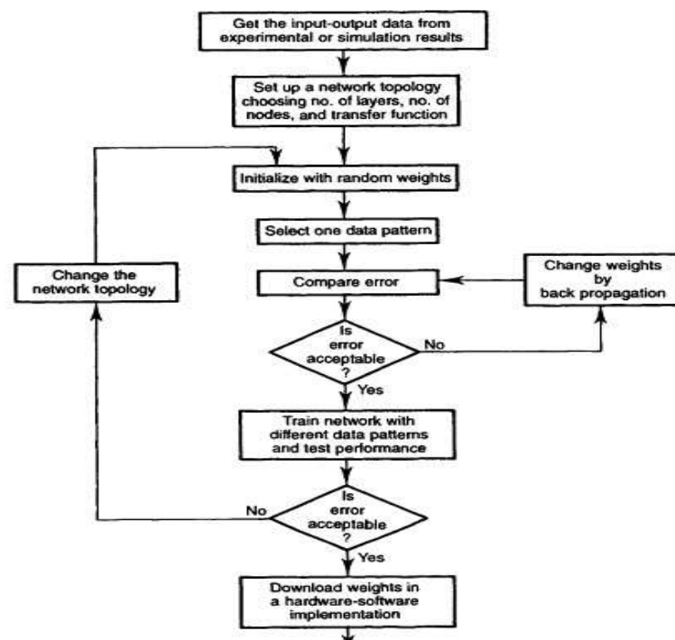
Figure 1. Flowchart for Training a Neural Network
