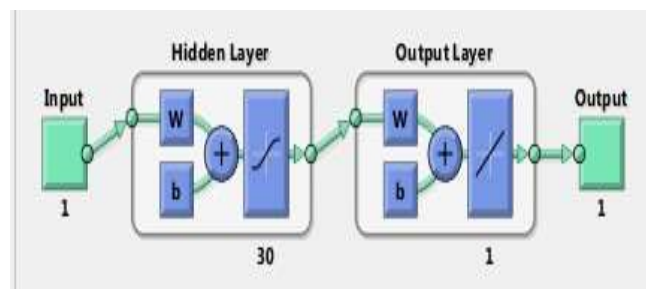
Figure 3. Custom Neural Network (Proposed Neural Network)
