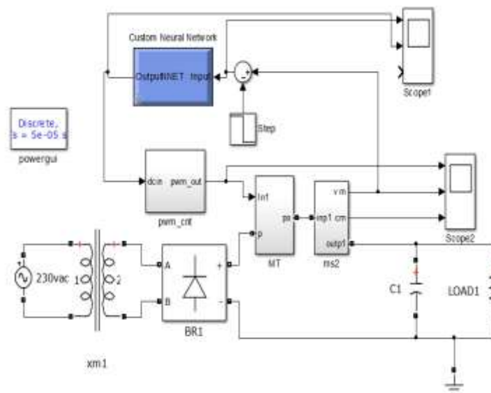
Figure 6. Neural Network Controller for AC-DC Power Converter Circuit
