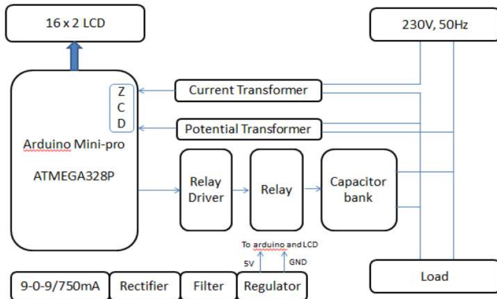
Fig B: Block Diagram of PFC using ATMEGA 328
