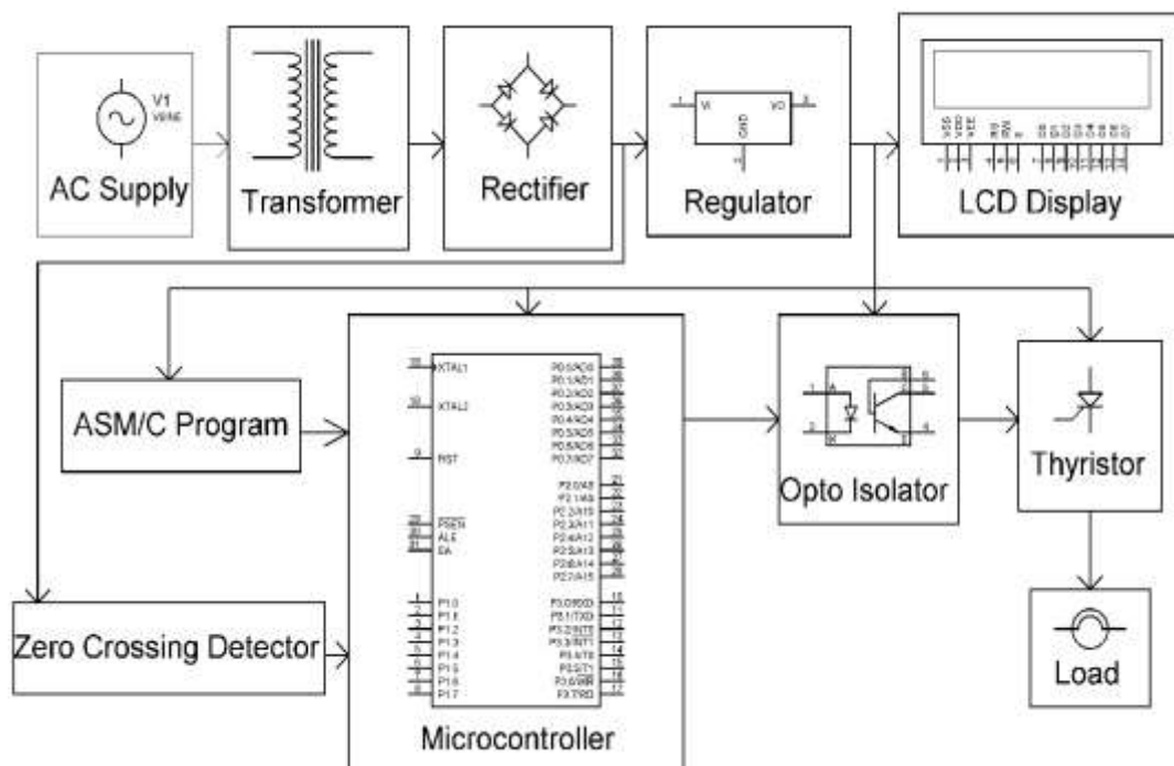
Fig 1:- Block Diagram
