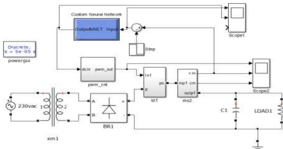
Figure 6. Neural Network Controller for AC-DC Power Converter Circuit
