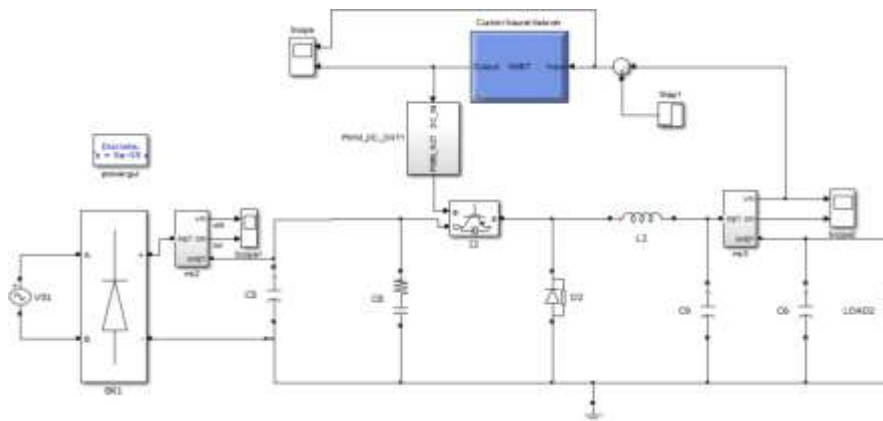
Figure 5. Neural Network Controller for DC-DC (Boost) Power Converter Circuit
