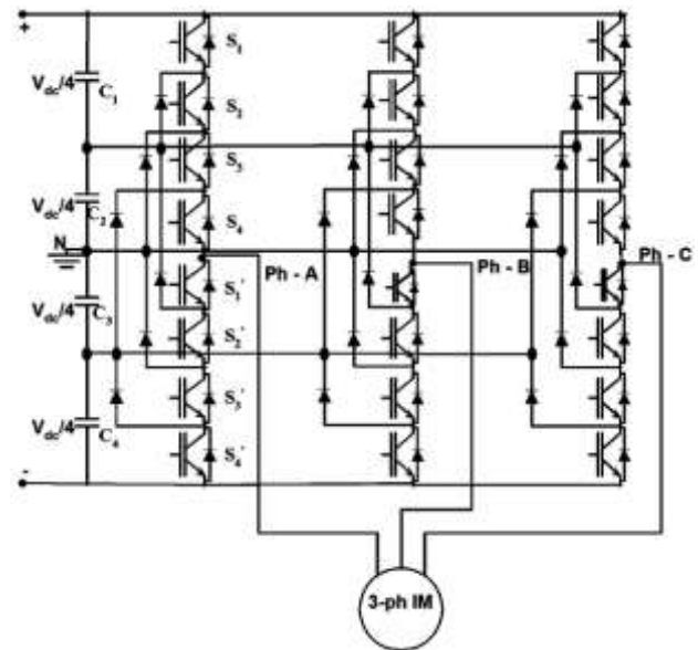
Fig.2. Multilevel inverter based drive circuit
