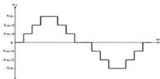
Fig.4. Three level inverter output voltage.
