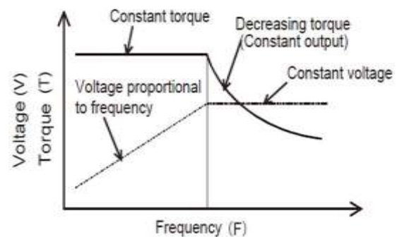
Fig.7. Speed-Torque characteristics with V/f control
