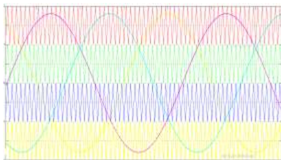
Fig.6. In-phase disposition technique
