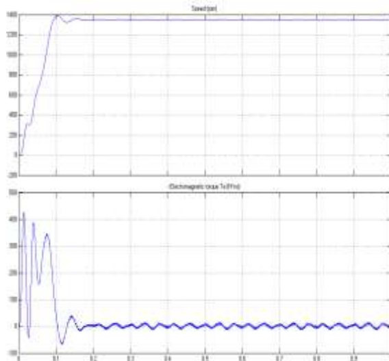
Fig.14. N-T curves for 45Hz frequency
