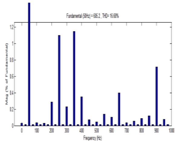
Fig.12. FFT for output voltage
