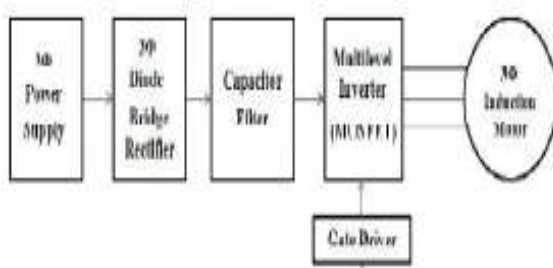
Fig.5. Basic block diagram
