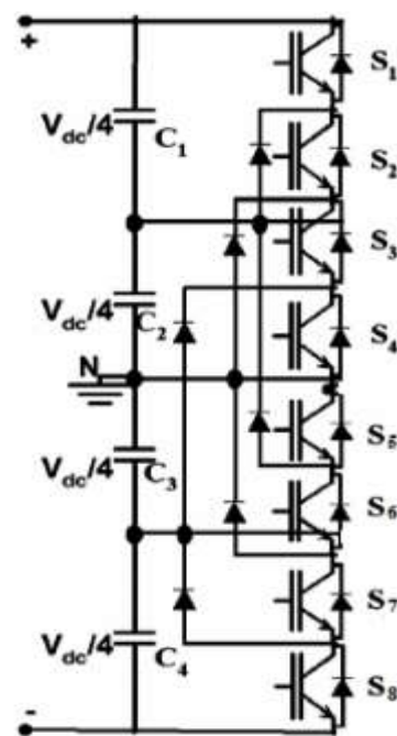
Single leg Diagram of Five level inverter
