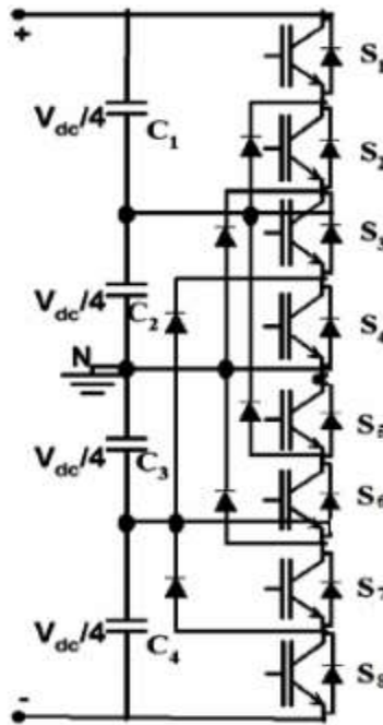
Single leg Diagram of Five level inverter
