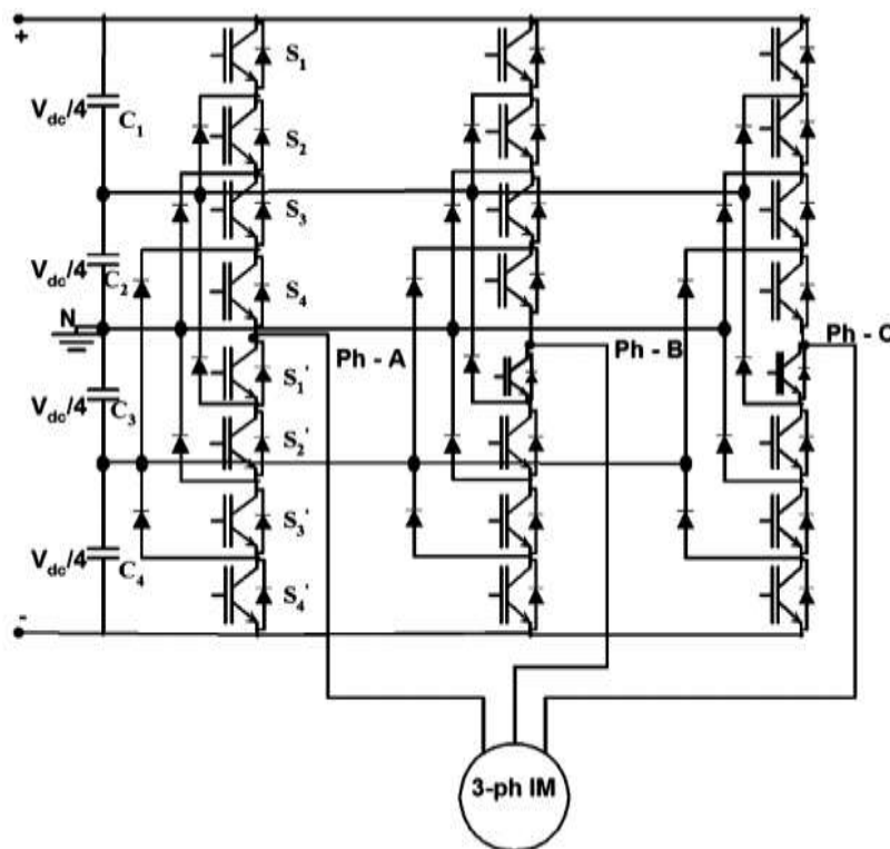
Fig.2. Multilevel inverter based drive circuit
