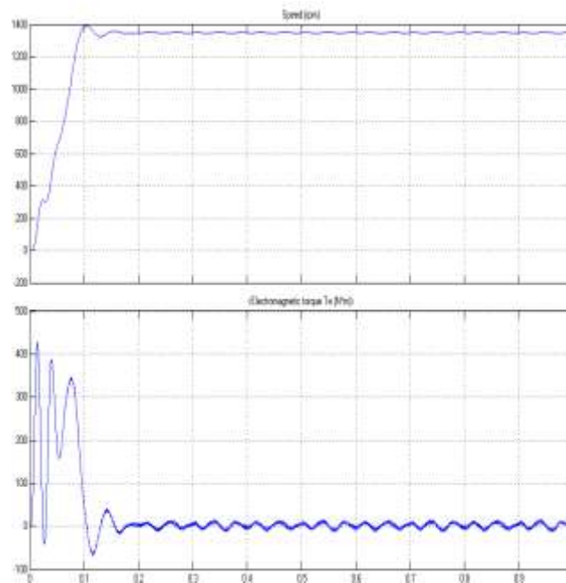
Fig.14. N-T curves for 45Hz frequency
