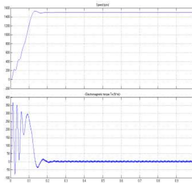
Fig.13. N-T curves for 50Hz frequency
