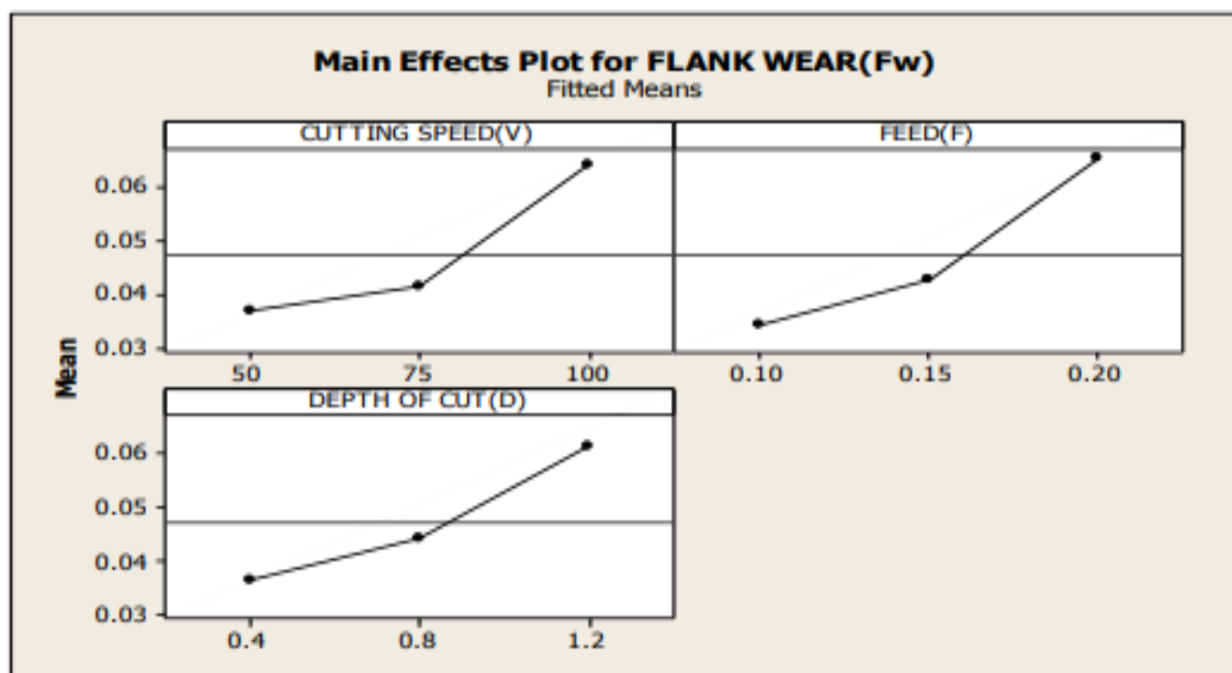
Fig: 3. Interaction plots for means of flank wear vs. parameters
