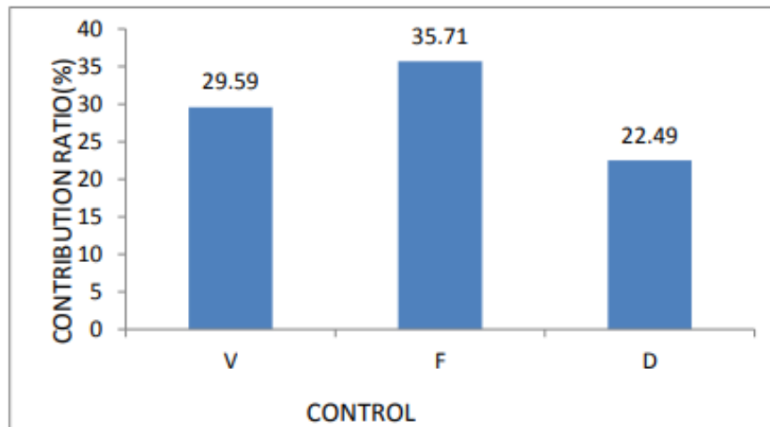
Fig: 4. Pareto Diagram for flank wear
