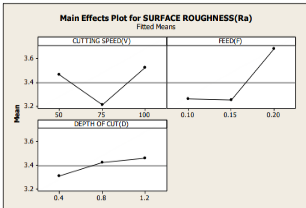
Fig: 1. Interaction Plots For Means of Surface Roughness vs. Parameters
