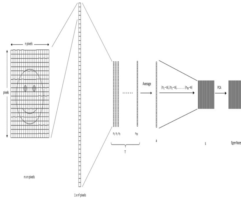
Fig.3.2. Splitting the Face
