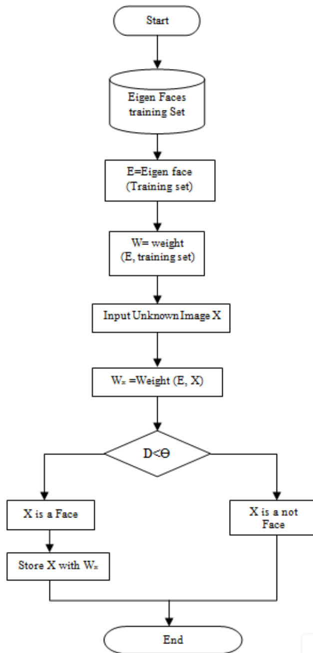
Fig.3.1. High-level functioning principle of the Eigenface-based facial recognition algorithm
