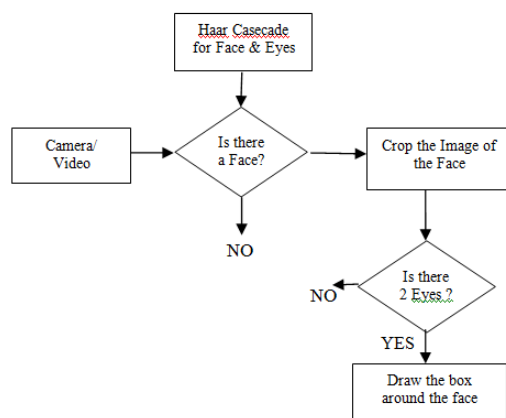
Fig. 2.1 Face detection flow operation
