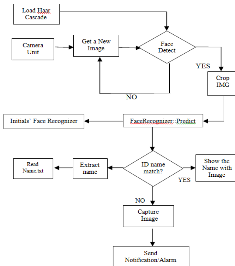
Fig.4.1. Face Recognition Flow chart
