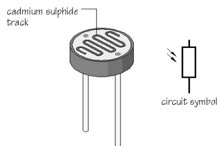
Fig. 4: Light Dependent Resistor
