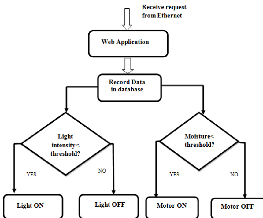
Fig. 6. Process flow for automation system
