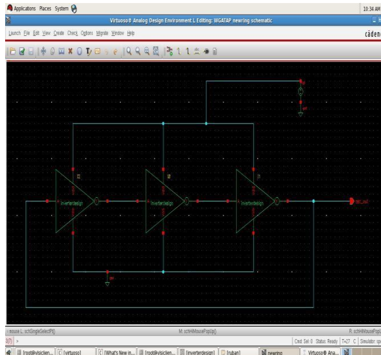
Figure 4.4 Ring Oscillators VCO
