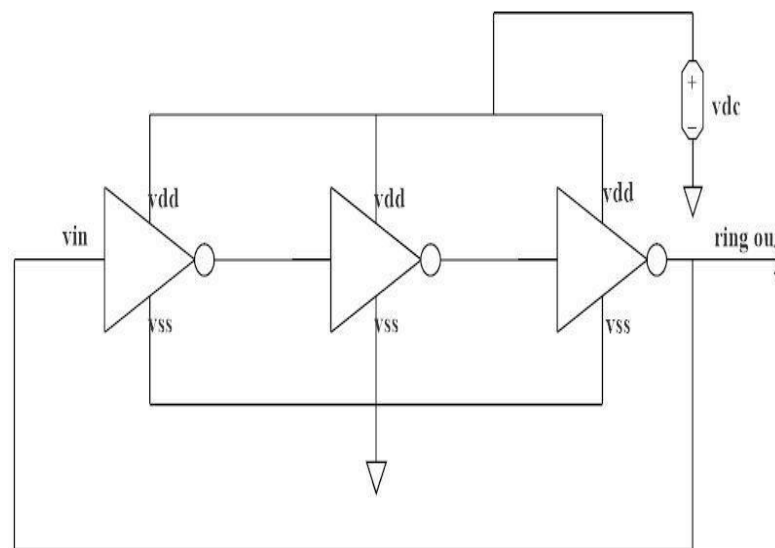
Figure 3.1 Schematic of Ring Oscillator
