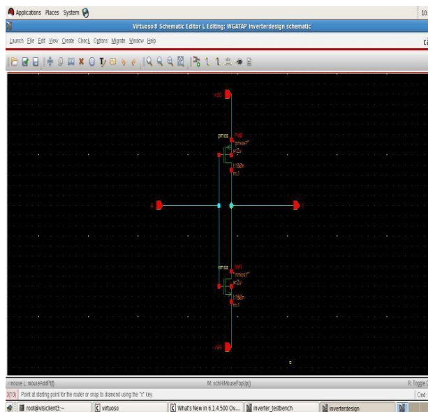
Figure 4.1 Schematic of a CMOS Inverter
