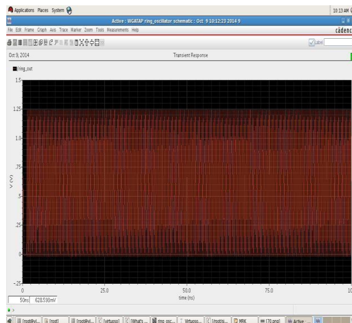
Figure 4.5 Transient response of Ring oscillator
