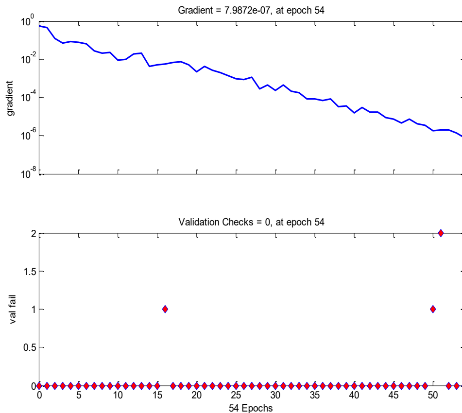
Fig 3 Training state of the network classifier
