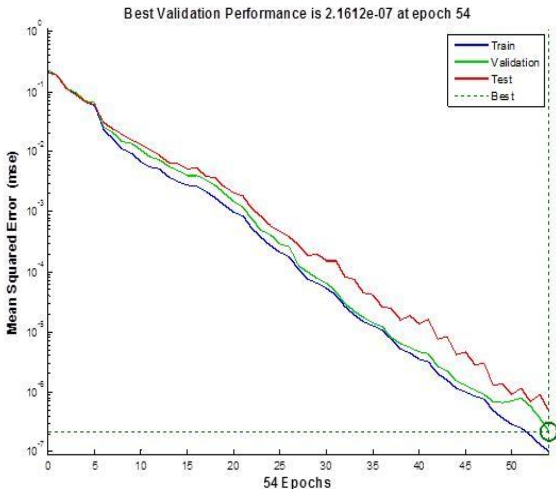
Fig 2: Performance of network classifier
