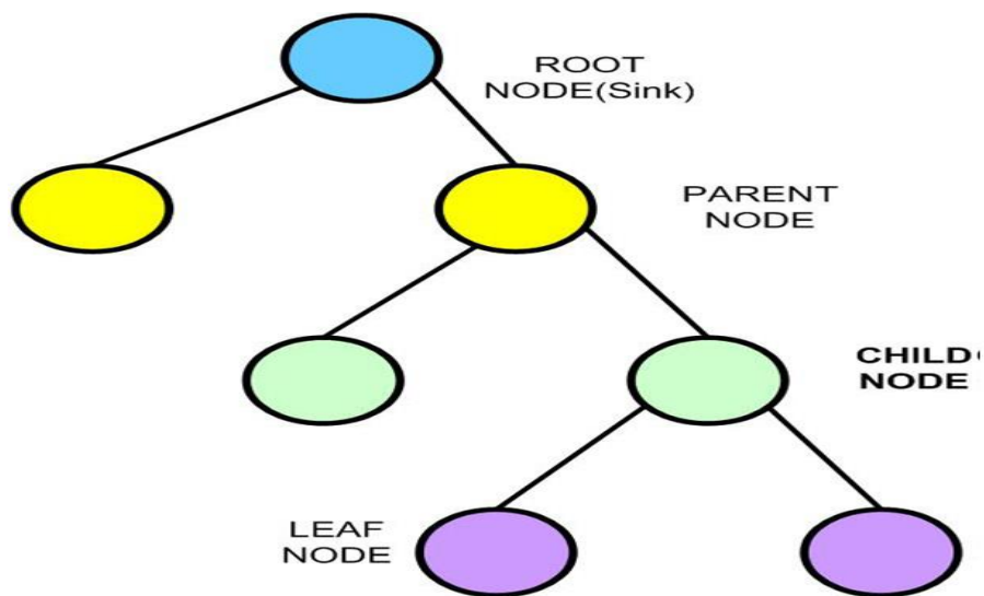
Figure 8: Tree-Based Approach
