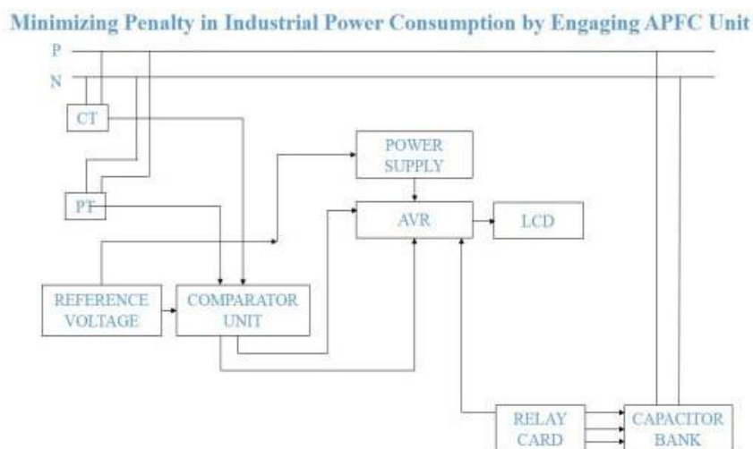
Fig -2: Block diagram of PFC using AVR microcontroller
