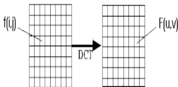
Fig.3. DCT blocks
