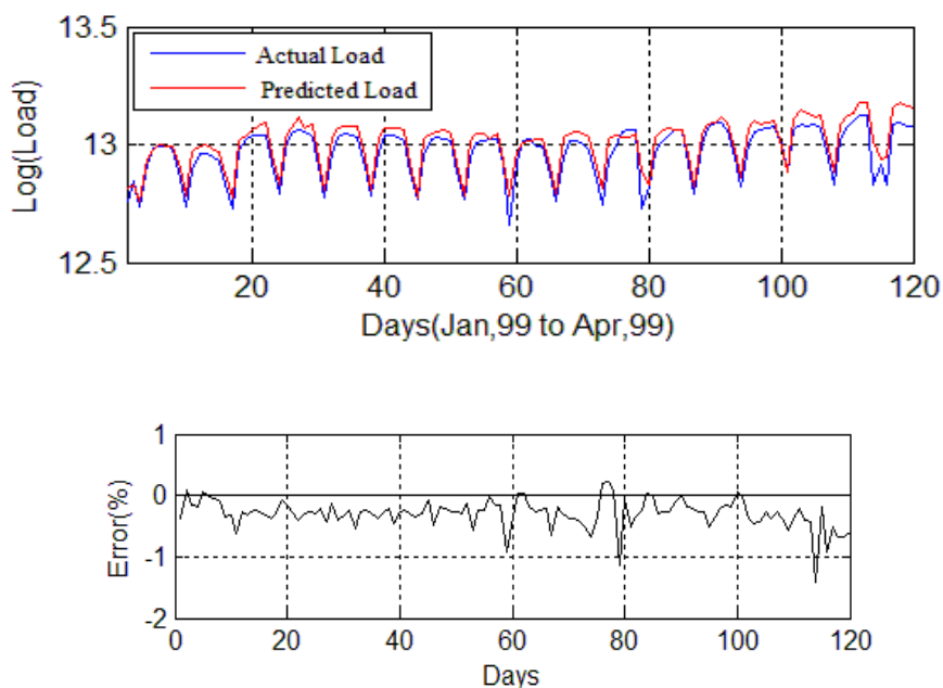
Fig. 4(a): Comparison between the actual load and the predicted load for 120 days obtained from standard model (SELF) used by feed forward neural network and (b): corresponding their errors in percentage.
