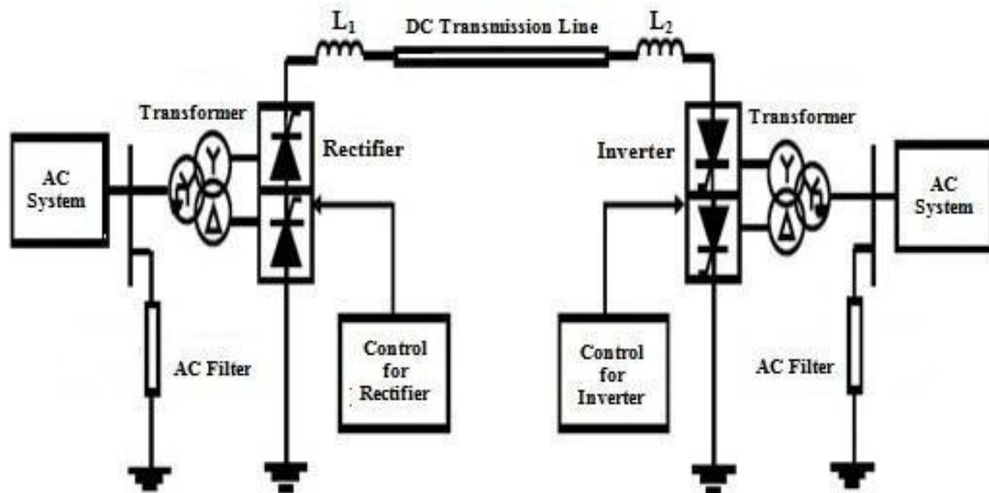
Figure1: The monopolar HVDC transmission system model
