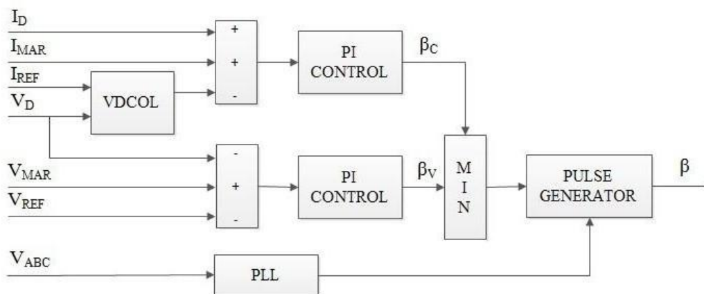
Figure3: Logic diagram of the inverter control system model.
