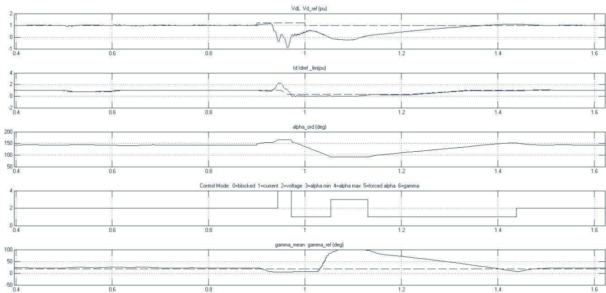
Figure5: Inverter DC quantities
