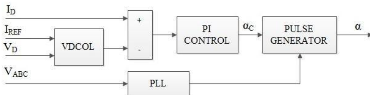
Figure2: Logic diagram of the rectifier control system model.
