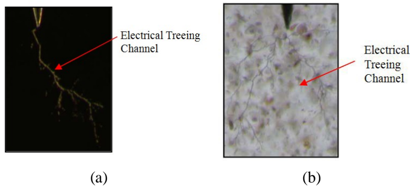
Fig. 5 Electrical tree initiation and propagation in silicone rubber (a) pure silicone rubber with tree initiated at 8.5kV and (b) silicone rubber with 1% EFB, tree initiated at 11kV
