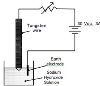
Fig. 1 Schematic diagram for the needle tip formation processes using Sodium Hydroxide (NaOH) solution
