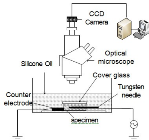
Fig. 3 Set-up of camera-equipped online monitoring system for electrical treeing studies schematic diagram
