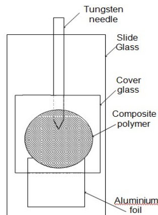
Fig. 2 Configuration of leaf-like specimen
