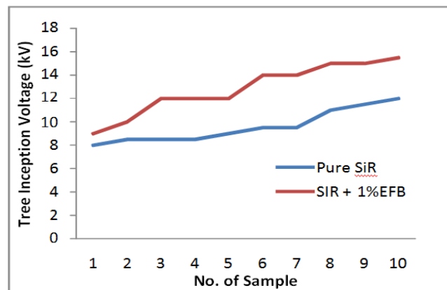
Fig. 4 Graphical view of Tree Inception Voltage for pure silicone rubber and silicone rubber with 1% EFB
