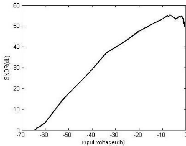
Fig. 10 Signal-to-Noise vs. input amplitude of the modulator
