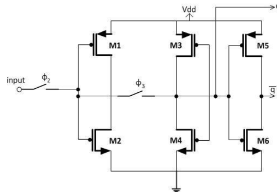
Fig. 7 Circuit diagram of D flip-flap
