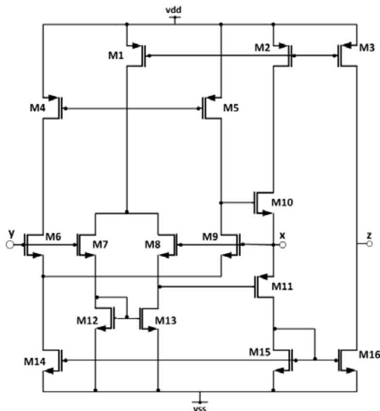
Fig. 3 Circuit diagram of the employed CCII
