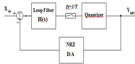
Fig. 1 Block diagram of a CT sigma-delta modulator
