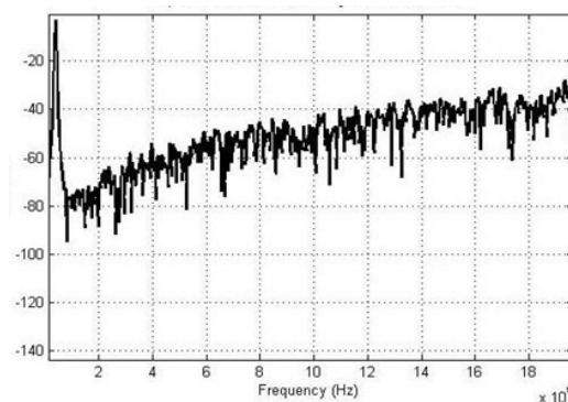
Fig. 9 Power spectrum of the modulator
