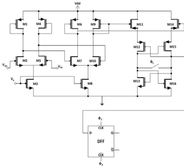
Fig. 6 Circuit diagram of the applied quantizer
