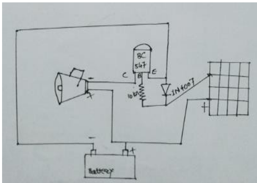
Fig 3.1 Block Diagram
