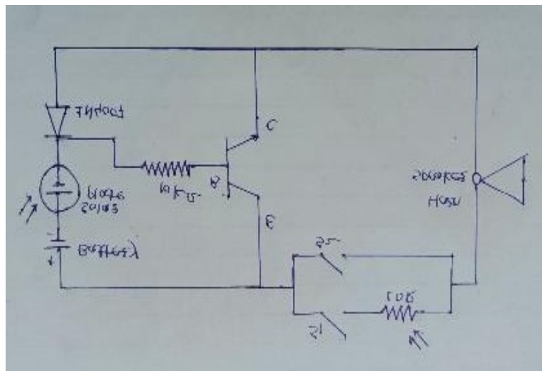
Fig 3.2 Circuit Diagram
