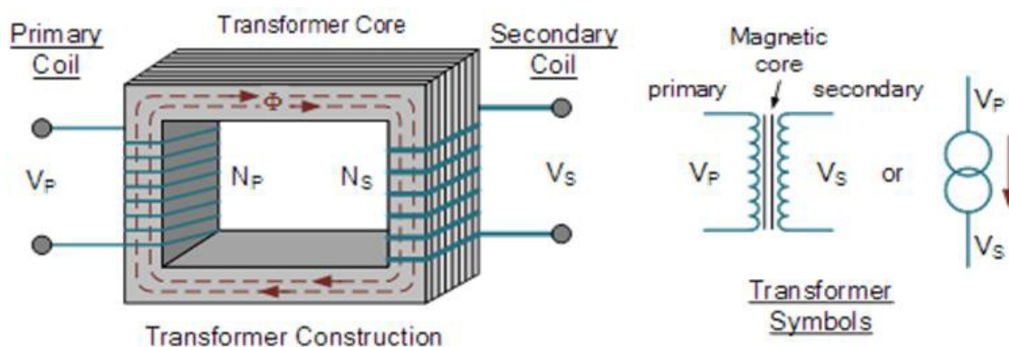
Figure 2: Transformer Construction (single-phase)
