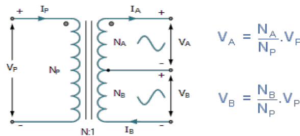
Figure 4: Transformer on center tapped diagram
