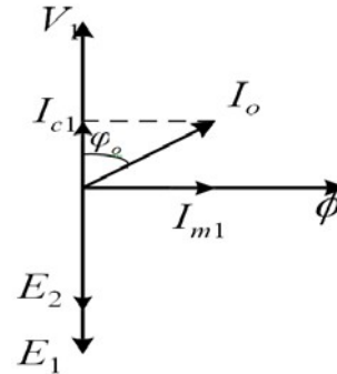
Figure 3: Transformer vector diagram
