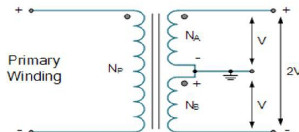
Figure 5: Center-tap Transformer using a Dual Voltage Transformer
