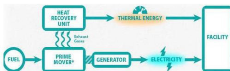
Fig 2 Topping Cycle
