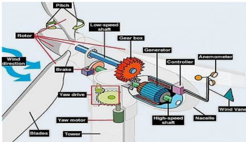
Fig-1 Horizontal wind turbine
