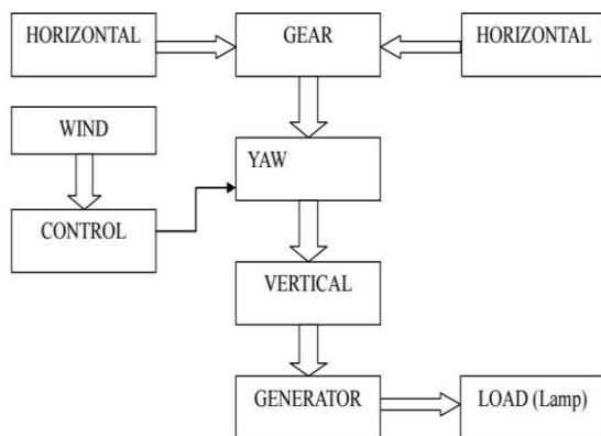
Fig-3 Proposed block diagram
