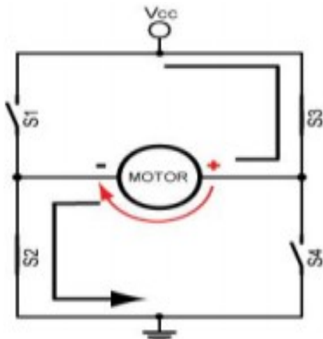
Fig 6: Motor Runs in “Reverse”(Switches 2 and 3 Closed)
