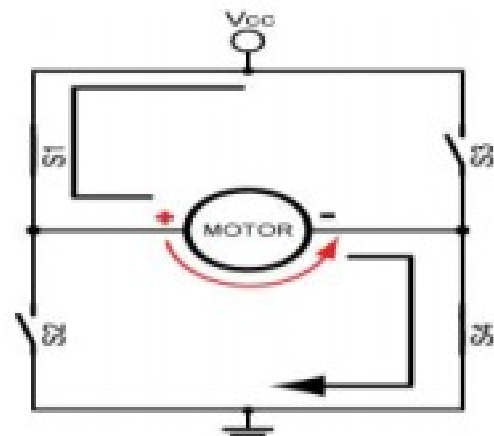
Fig 5: Motor Runs "Forward"(Switches 1 and 4 Closed)
