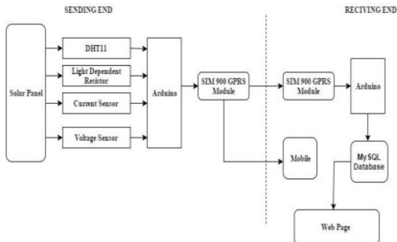
Fig 7: Block Diagram of Proposed Methodology
