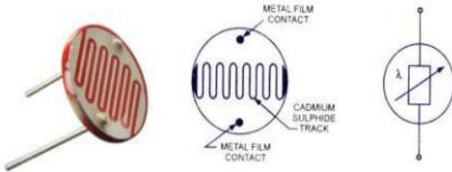
Fig 4: Light Dependent Resistor (LDR)
