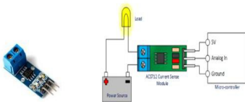
Fig5: Current Sensor (ACS712) and connection with Arduino-UNO
