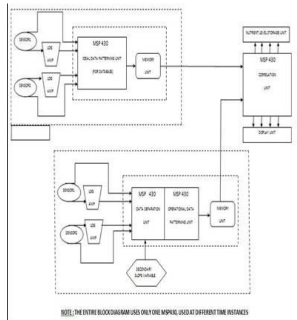
Figure 1: Block Diagram
