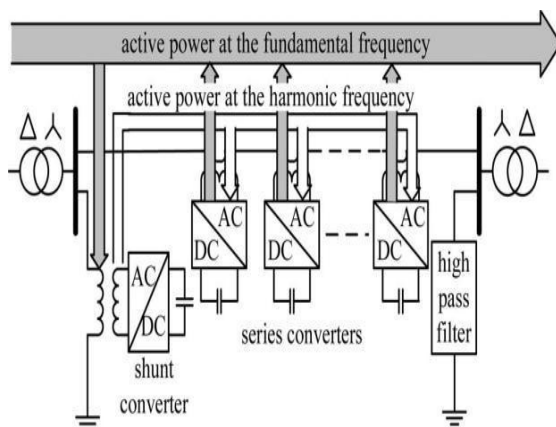
Fig. 3: DPFC configuration.
