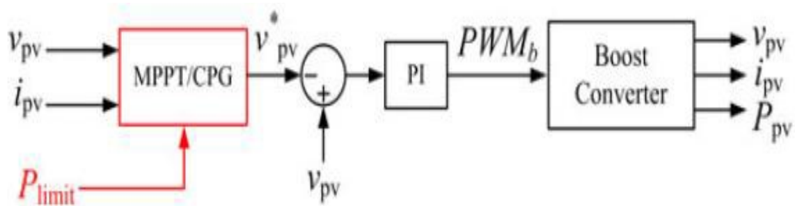
Fig. 5 Control structure of the Perturb and Observe based CPG algorithm (P&O-CPG), where a Proportional Integrator (PI) is adopted.
