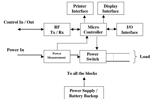
Figure 6: Customer Premises Equipment (Slave unit)
