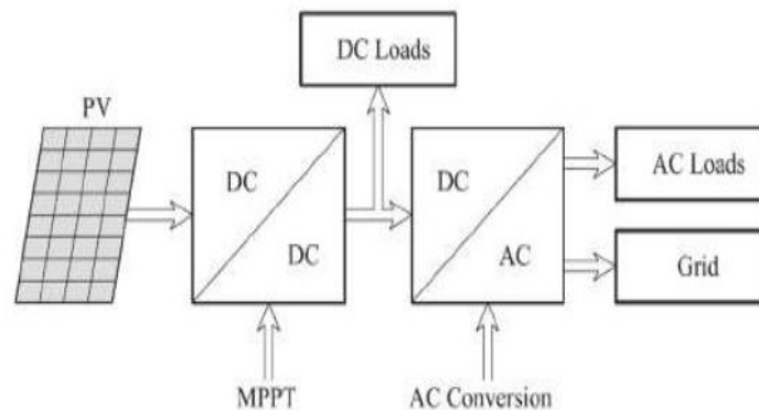
Fig 2: Basic Block Diagram of MPPT
