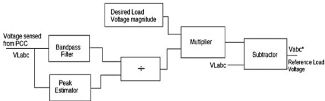
Fig.2 Block diagram for control of series active filter
