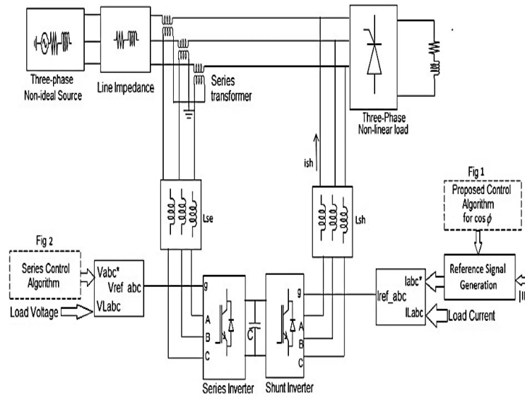
Fig. 3 Simulation model of test system with UPQC
