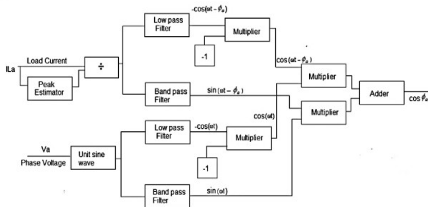
Fig. 1 Schematic of proposed control algorithm for extracting \cos\phi for phase a
