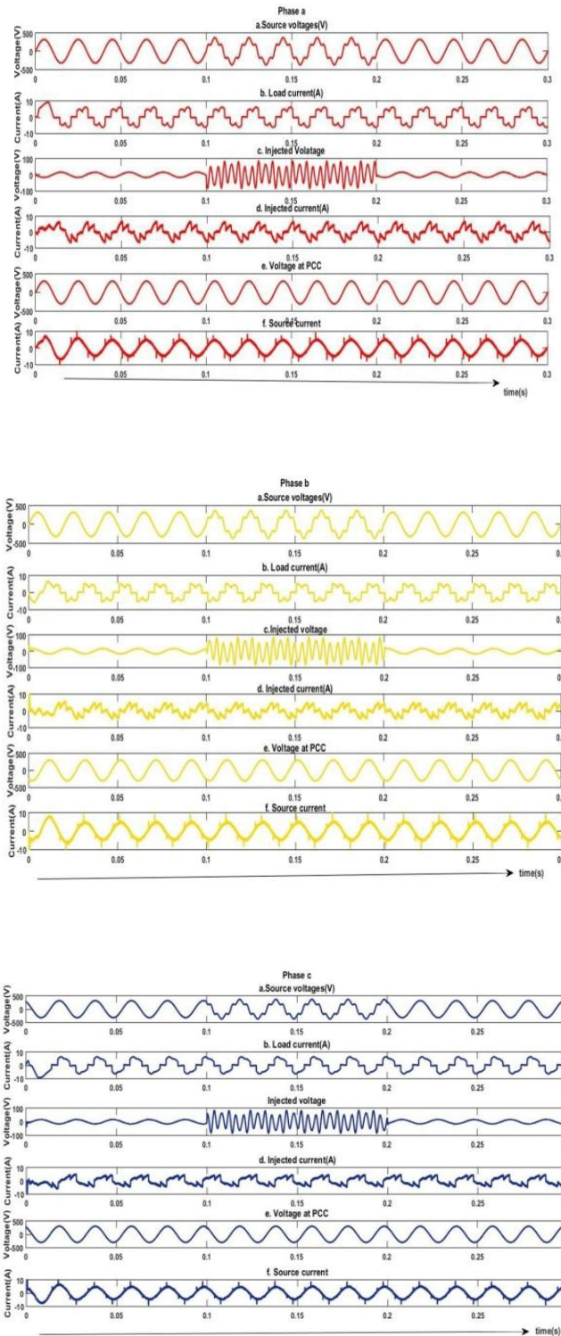
Fig. 4. Simulation results of (a) source voltage,(b) load current,(c) series injected voltage,(d) shunt injected,e) voltage with UPQC at PCC, (f) source current for a thyristor converter feeding a RL load with distorted supply and balanced load condition.
