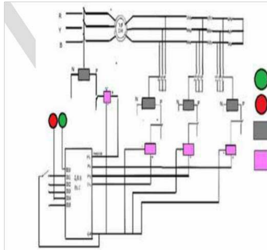
Figure 3: Panel board circuit
