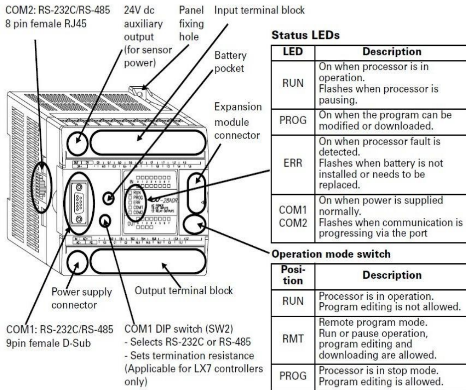
Figure 2-Internal structure of plc LX7
