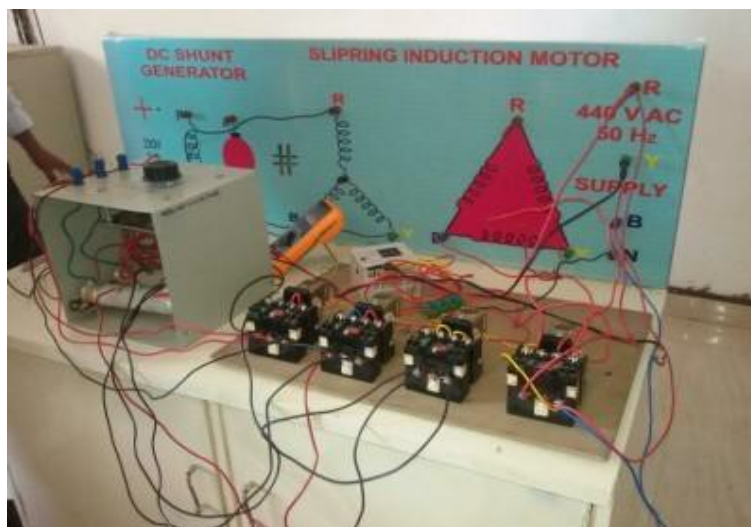
Figure 4: Panel board design
