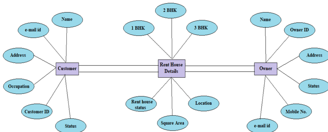
Figure 9. An ER diagram showing the working of Rental House
