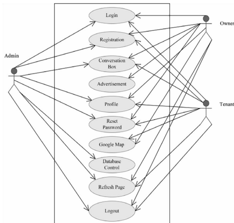
Figure 8. Total use case diagram of the Rental House Management System
