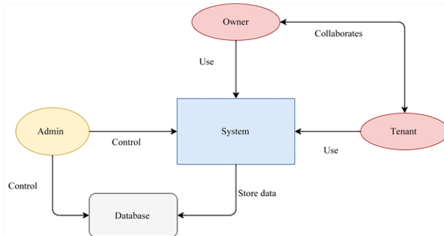
Figure 7. Basic use case diagram showing how the Rental House Management System works
