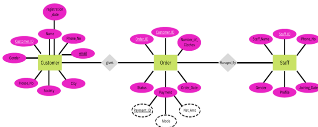
Figure 9. Entity Relationship Diagram
