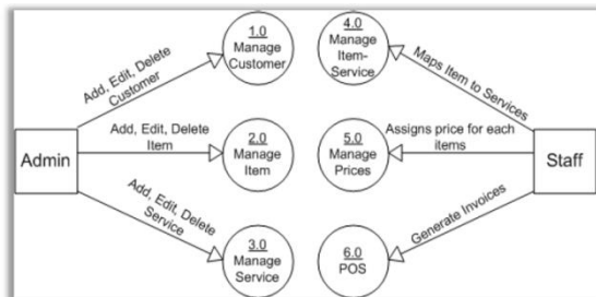
Figure 12. Level 1 Data Flow Diagram
