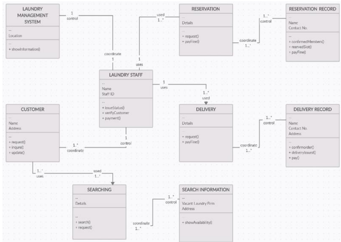
Figure 10. Class Diagram
