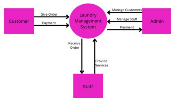
Figure 11. Level 0 Data Flow Diagram
