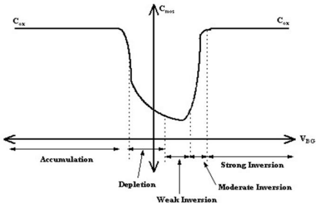
Fig.4. Capacitance versus voltage characteristics
