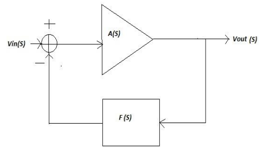
Fig.1. Negative feedback system with frequency selective network
