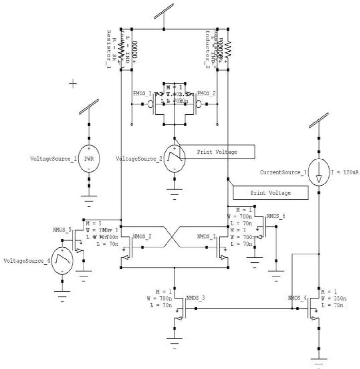
Fig.5. Proposed cross coupled differential LC VCO topology.
