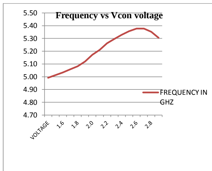
Fig.7. Frequency vs. vcon voltage plot
