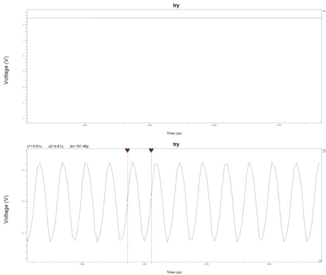
Fig.6. Simulation result of Proposed crossed coupled differential LC VCO topology
