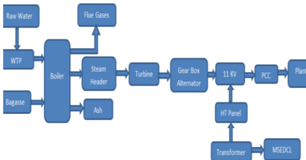
Fig 4 Block Diagram of Co-generation Project
