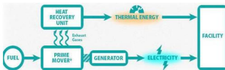
Fig 2 Topping Cycle
