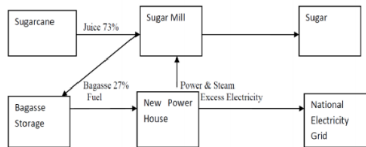
Fig1. Principle of cogeneration
