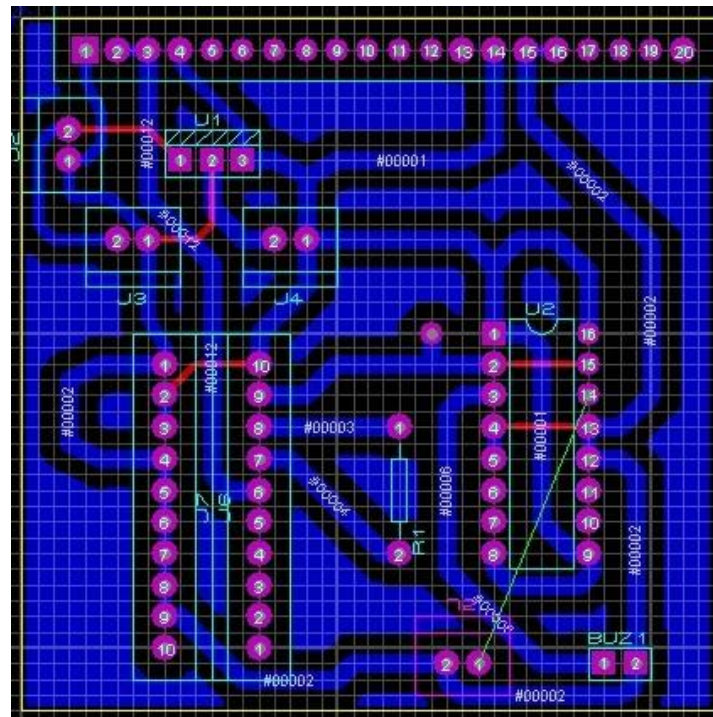
Fig 7 Receiver PCB Layout
