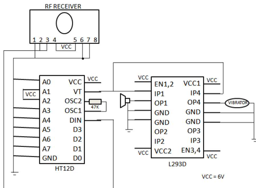
Fig 5 Receiver circuit diagram (with address "01100000")
