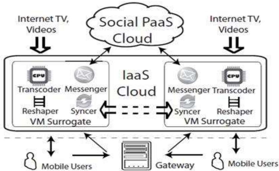
Figure:1 The architecture of CloudMoV
