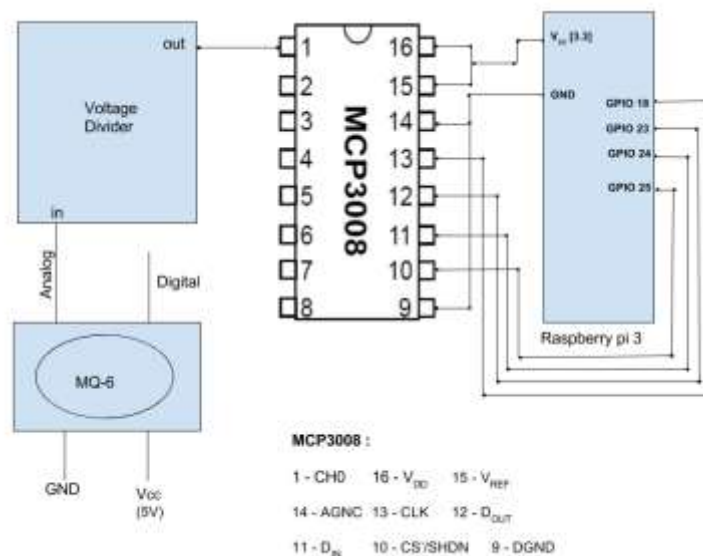
Fig.4: Circuit Connections for AAGLN
