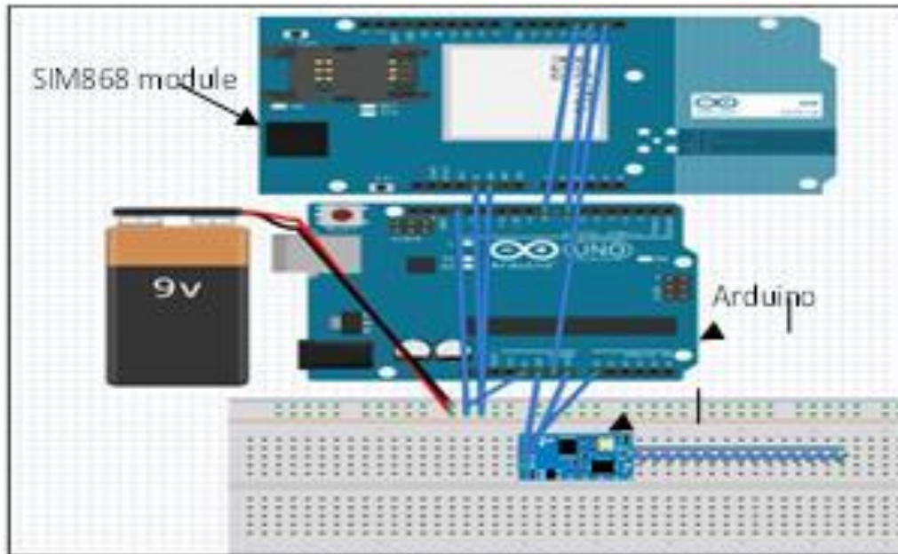
Fig. 3: The design of the circuit using Fritzing software
