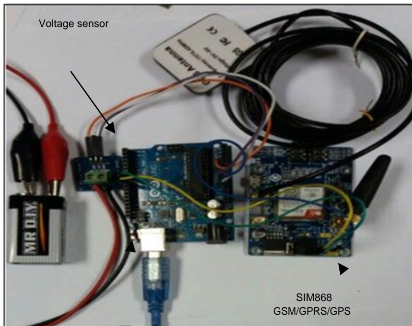
Fig. 4: The actual design of the hardware for the proposed battery management system
