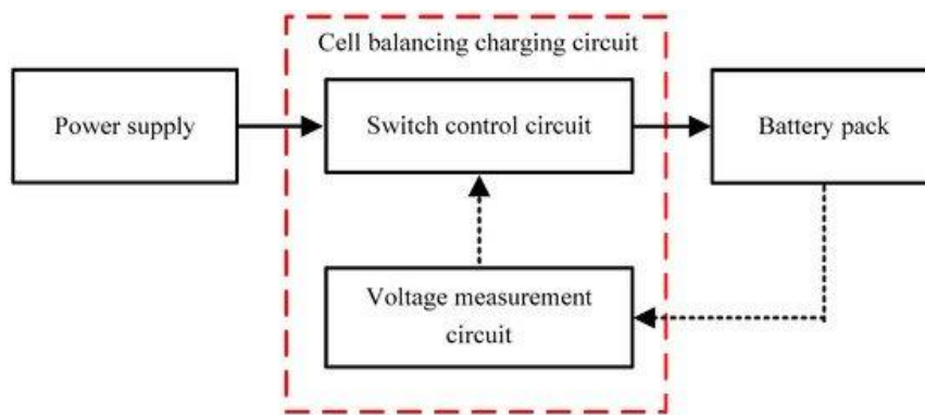
Fig. 9: Cell balancing Mechanism
