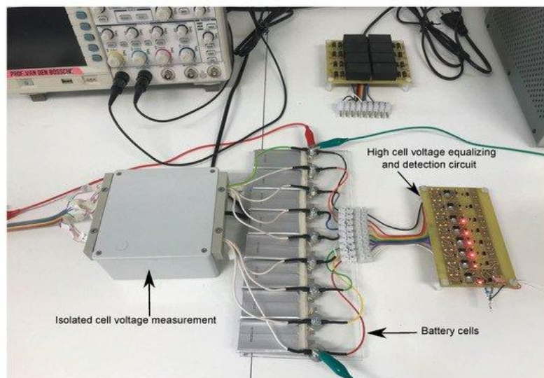
Figure 12: Hardware Implementation of cell balancing mechanism for an IOT enabled BMS in EV
